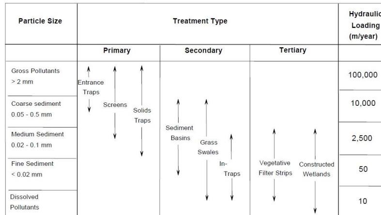
Figure 11: Linear relationship between contaminate particle size and level of treatment required for its effective removal (Perrrens Consultants, 2003)
